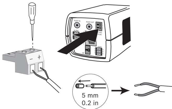
Figure 5.5 Power connection
